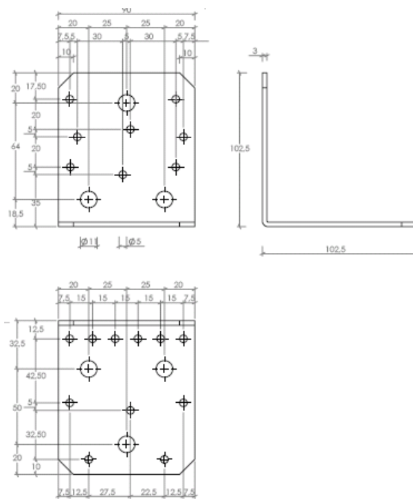
Figure A.3 Dimensions of Angle Bracket 6145
